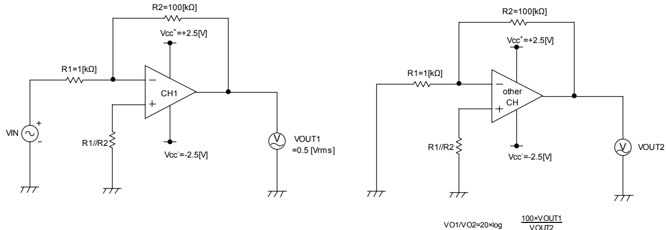
Fig.5 Measurement Circuit3
